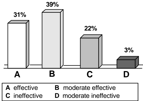
Fig.6: System evaluation.
