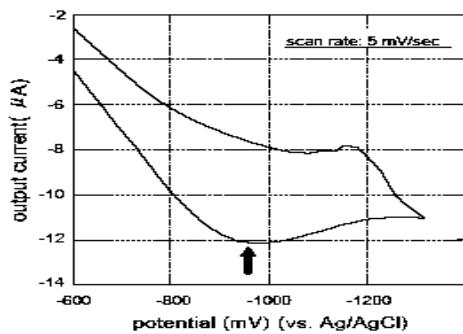
Fig. 5 Cyclic voltammogram of the ITO electrode (Sweep range: 0-1000 mV, scan rate: 5 mV/sec).
