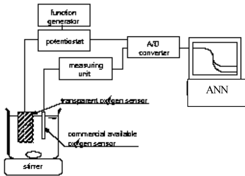
Fig. 4. Schematic diagram of the cyclic voltammeter of the transparent electrode.
